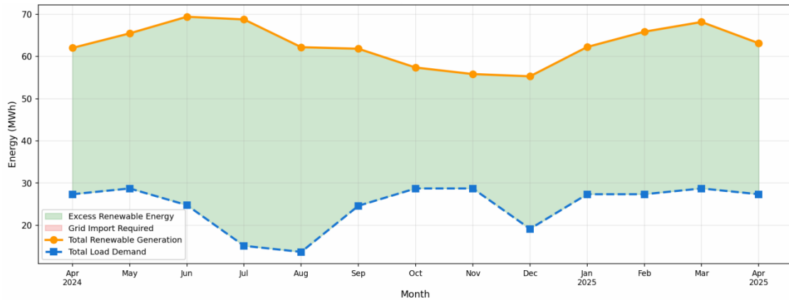
Figure 11: Monthly Energy Balance - Renewable Generation vs Load Demand (Annual Excess: 122,840 kWh | Annual Grid Import: 282,930 kWh)
