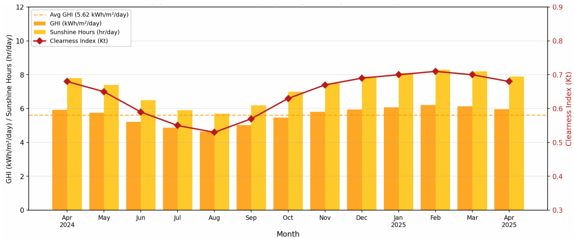
Figure 3: Monthly Solar Irradiance, Sunshine Hours and Clearness Index (Ajayi Crowther University, Oyo, Nigeria - Apr 2024 to Apr 2025)
