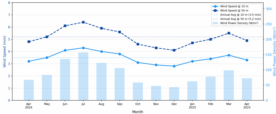
Figure 2: Monthly Wind Speed and Power Density Profile (Ajayi Crowther University, Oyo, Nigeria - Apr 2024 to Apr 2025)
