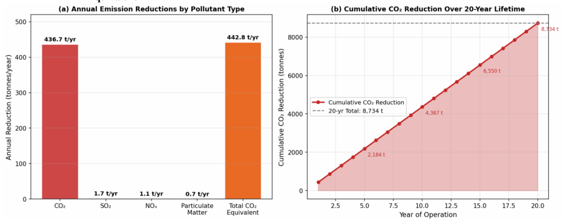
Figure 13: Environmental Impact - Annual and Cumulative Emission Reductions
