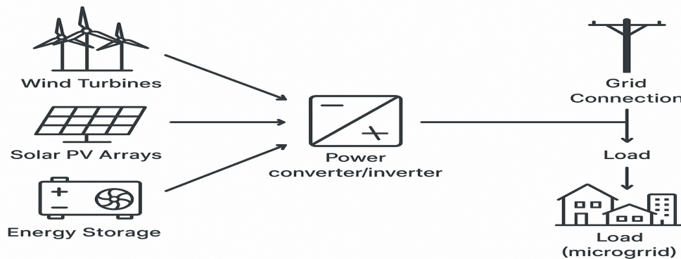
Figure 5: System Architecture
