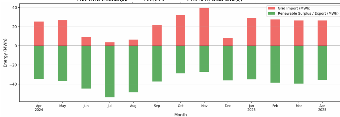
Figure 12: Monthly Grid Exchange - Import and Renewable Surplus (Annual Import: 282,930 kWh | Annual Export: 122,840 kWh)
