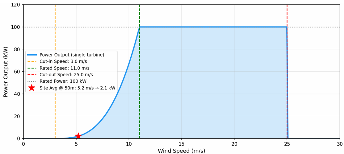
Figure 6: Wind Turbine Power Curve (100 kW PMSG, C_p = 0.42 ) with Site Annual Average Wind Speed Indicated
