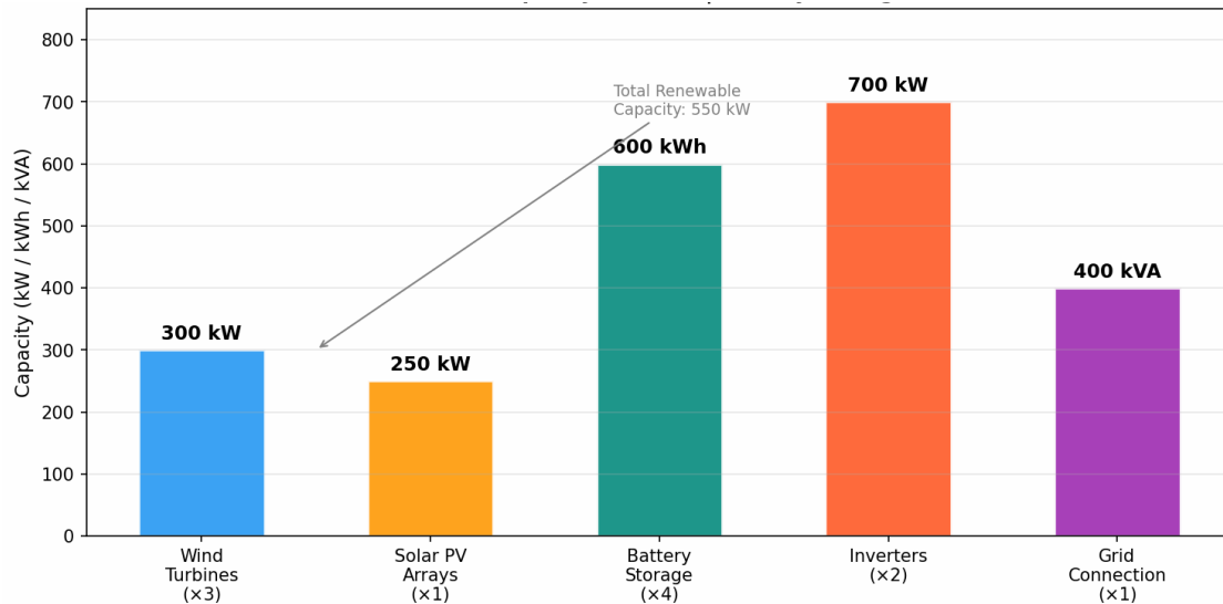
Figure 4: Installed System Component Capacities (Total Renewable Capacity: 550 kW | Battery Storage: 600 kWh)
