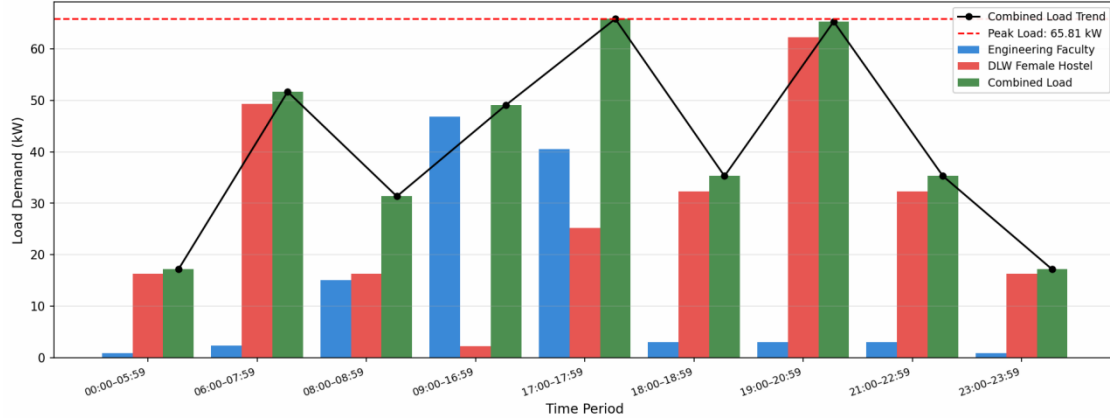
Figure 7: Hourly Load Demand Profile - Engineering Faculty and DLW Female Hostel (Peak Combined Load: 65.81 kW at 17:00-17:59)
